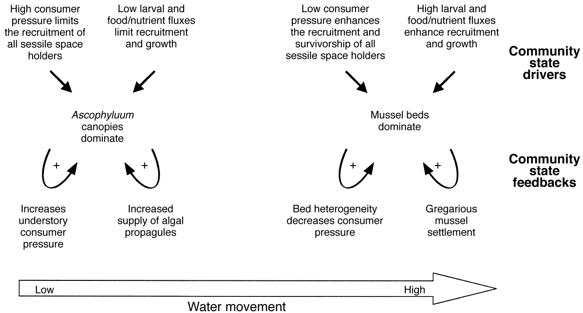
FIG. 10. Conceptual model of the deterministic generation and maintenance of Ascophyllum canopy–mussel bed alternate community states on Gulf of Maine rocky shores. At low-flow sites, intense consumer pressure by snails and crabs leads to habitats dominated by an unpalatable seaweed canopy, whereas at high-flow sites, low consumer pressure and high recruit supply lead to mussel bed habitats. Positive feedbacks in each community type lead to its expansion and persistence. If stochastically determined alternate stable states occur in this system, they are predicted to occur at intermediate-flow sites where consumer control and the predictability of larval recruitment are relaxed.
